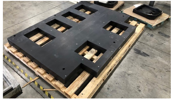
Multi-Cavity
